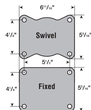
Alternative ISO Top Plates
