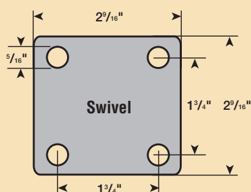
Standard Top Plates
