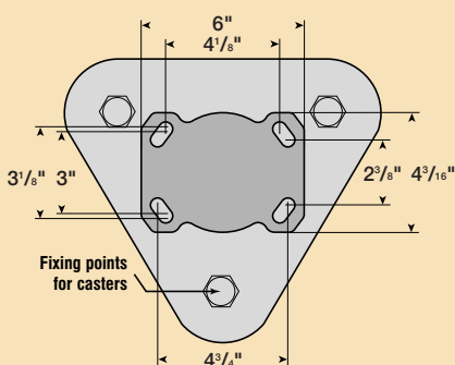
Standard Top Plate
